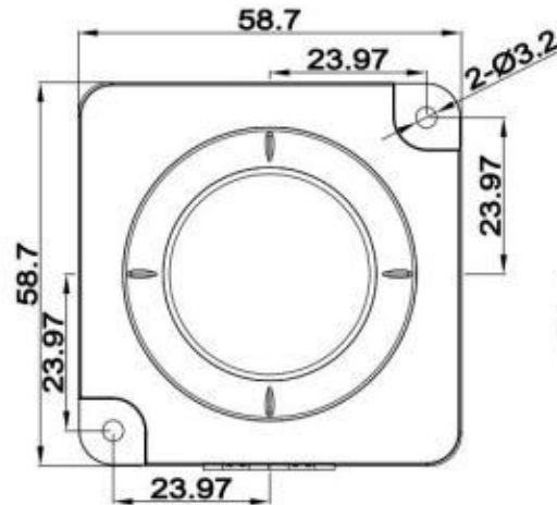
Front installation dimension drawing
