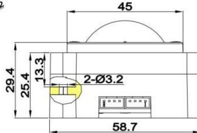
Side installation dimension drawing
